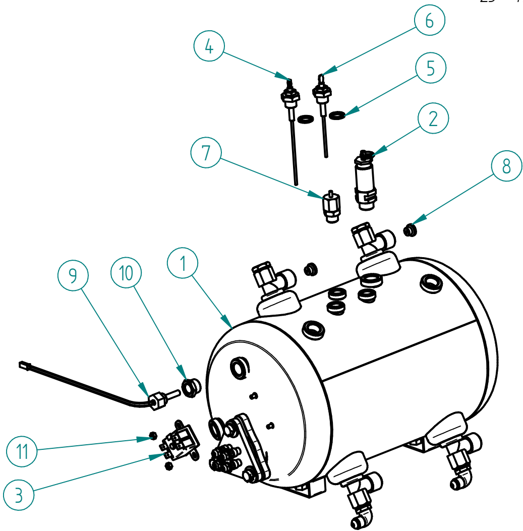
1 – 7.0.000.0533 – CALDEIRA 2GR 11 LT C/ ACESS. 1 – 2 GROUP 11 LT BOILER W/ ACESS.
