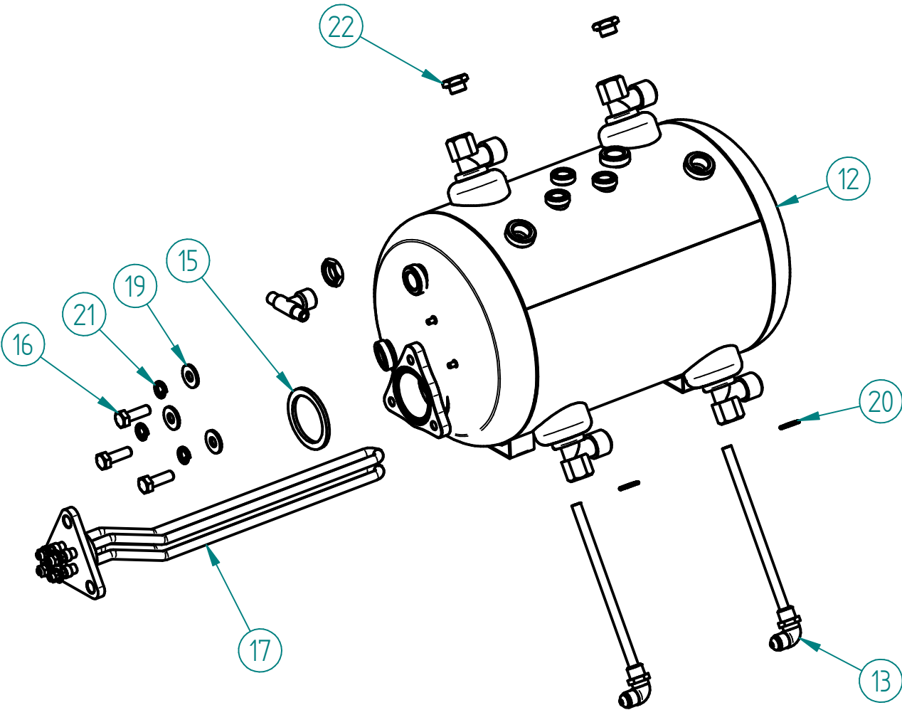
1 – 7.0.000.0533 – CALDEIRA 2GR 11 LT C/ ACESS. 1 – 2 GROUP 11 LT BOILER W/ ACESS.
